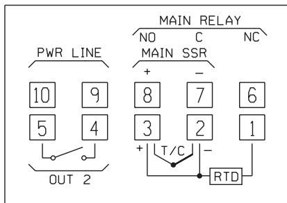
Fig. 3 POWER LINE WIRING
