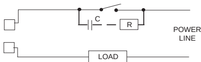
Fig. 7 EXTERNAL SWITCH IN SERIES WITH THE INTERNAL CONTACT
