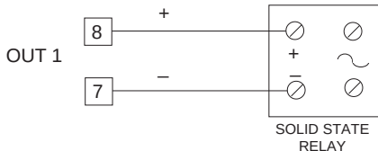
Fig. 8 SSR DRIVE OUTPUT WIRING
