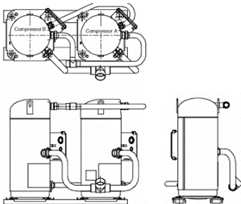
Figure 5: Tandem configurations
